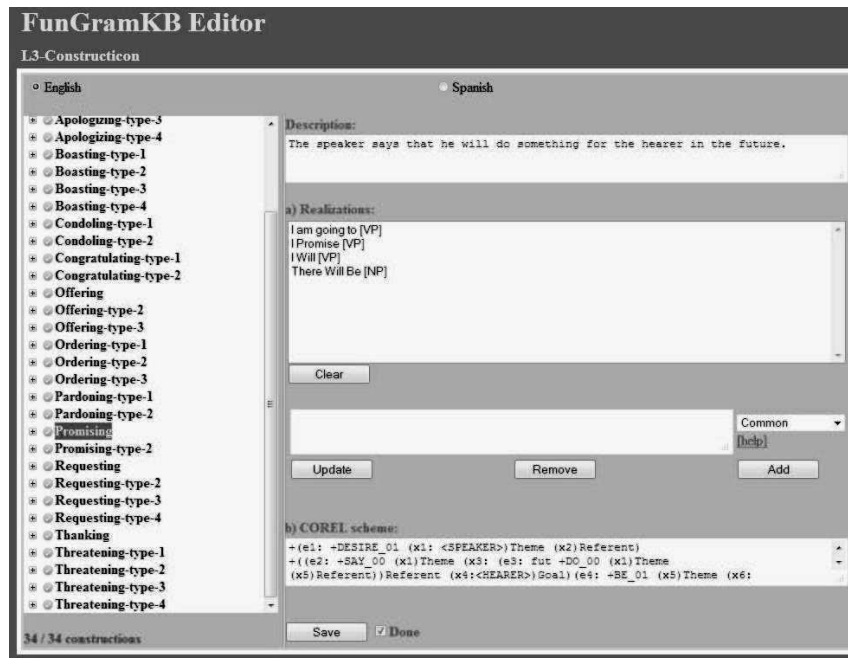
Figure 9: Interface of the Level-3 construction Promising .
