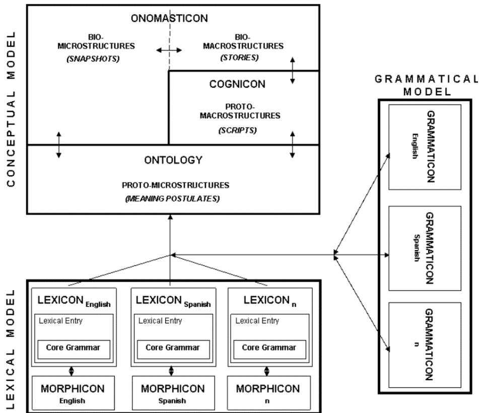
Figure 2: The FunGramKB architecture (reproduced from Perinián-Pascual and Mairal, 2012: 335).
