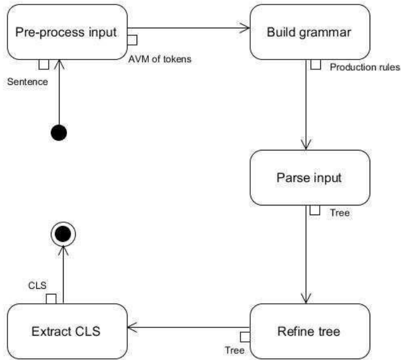
Figure 4: The architecture of ARTEMIS (Periñán-Pascual & Arcas, 2014).
