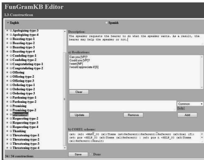
Figure 8: Interface of the Level-3 construction Requesting .
